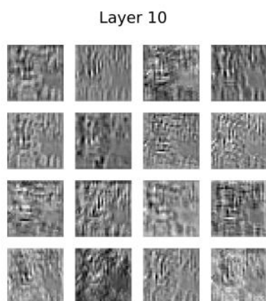
Figure 2.17: Select few feature maps in the 10th layer of ResNet18 [33] trained on ImageNet [77].
