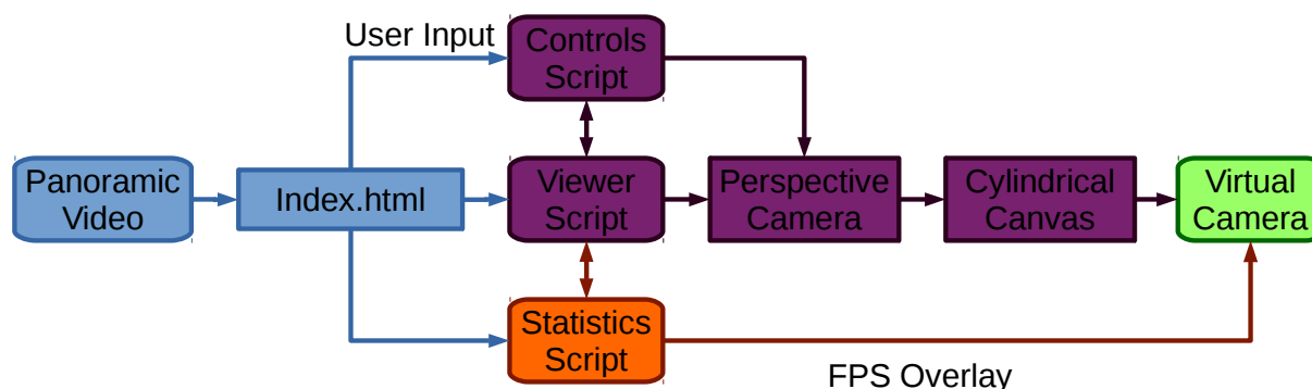
Figure 4.1: WebGL-based panoramic video viewer prototype architecture
