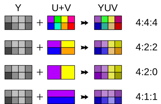
(b) YUV chroma sub-sampling schemes
