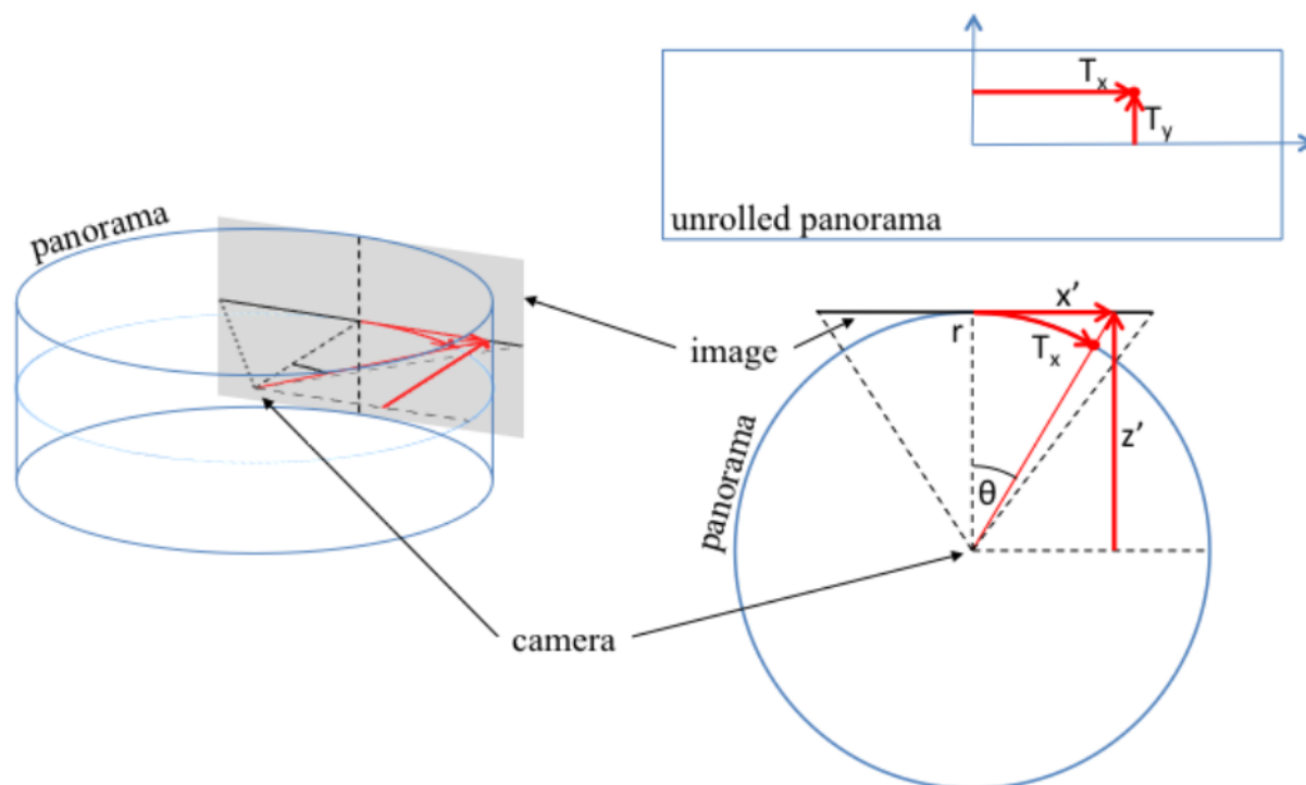
Figure 2.8: Mapping pixels from a captured image to panorama
