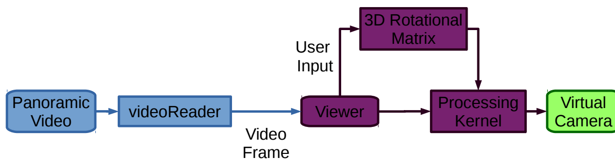
Figure 3.2: Panorama viewer prototype architecture
