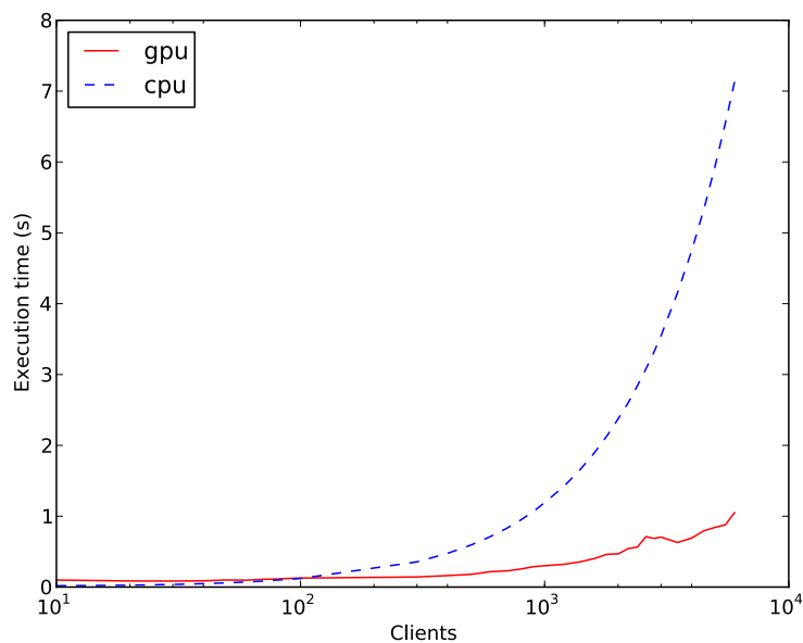
Figure 3.19: Execution time (in seconds) of the cheat detection mechanism on the GPU and the CPU.
