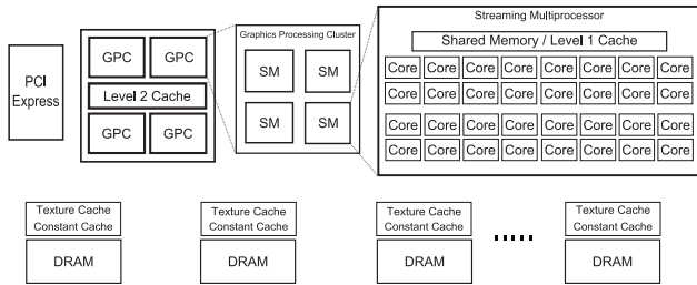
Figure 1. Nvidia GF100 Compute Architecture
