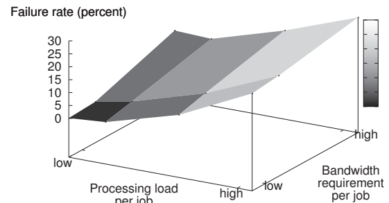
Figure 3: Failure rate versus processing and communication costs (FF on nVidia G84)
