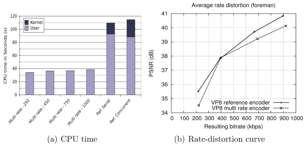
Figure 3. CIF streaming scenario foreman
