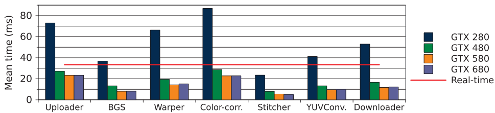
Fig. 15. GPU comparison.
